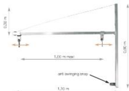
Ref: PIX01 H:0,80 m - L: 1,10 m - inter distance max: 1,00 m - max load: 25 kg
